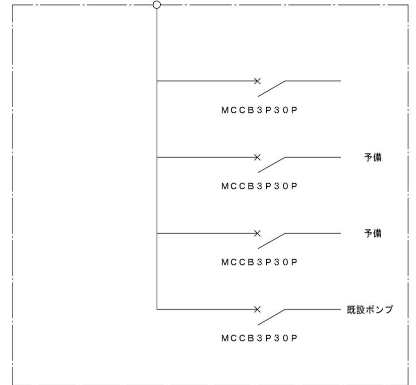
既設動力盤 (1LM-2)
